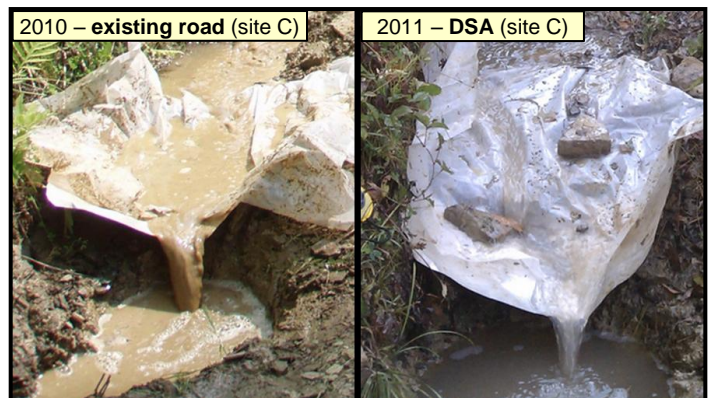
The runoff collection point from site “C” is shown here for both the “existing” road in 2010, and after DSA placement in 2011 showing a 95% sediment reduction.
