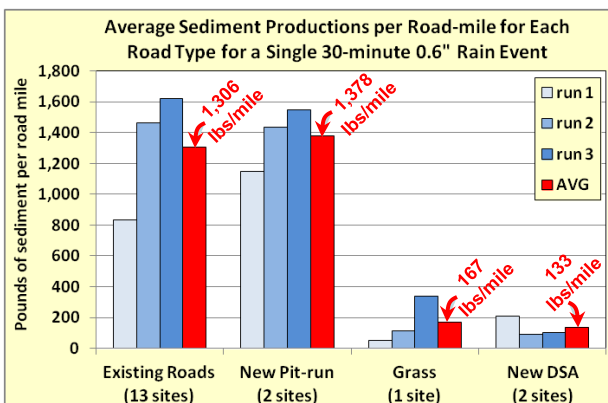
Average sediment production per road-mile by road type. Note the number of test sites available for use in averages varies from 1 to 13.
